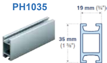
37" Beam
