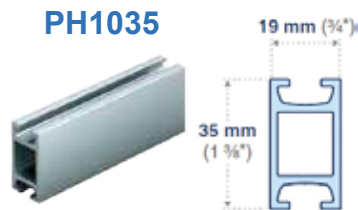
27½" Beam
