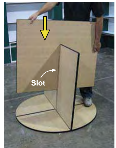
Leg with slot facing down
