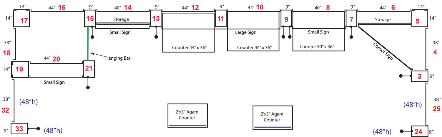
TOP VIEW Floor Plan A2: 10'x30'
