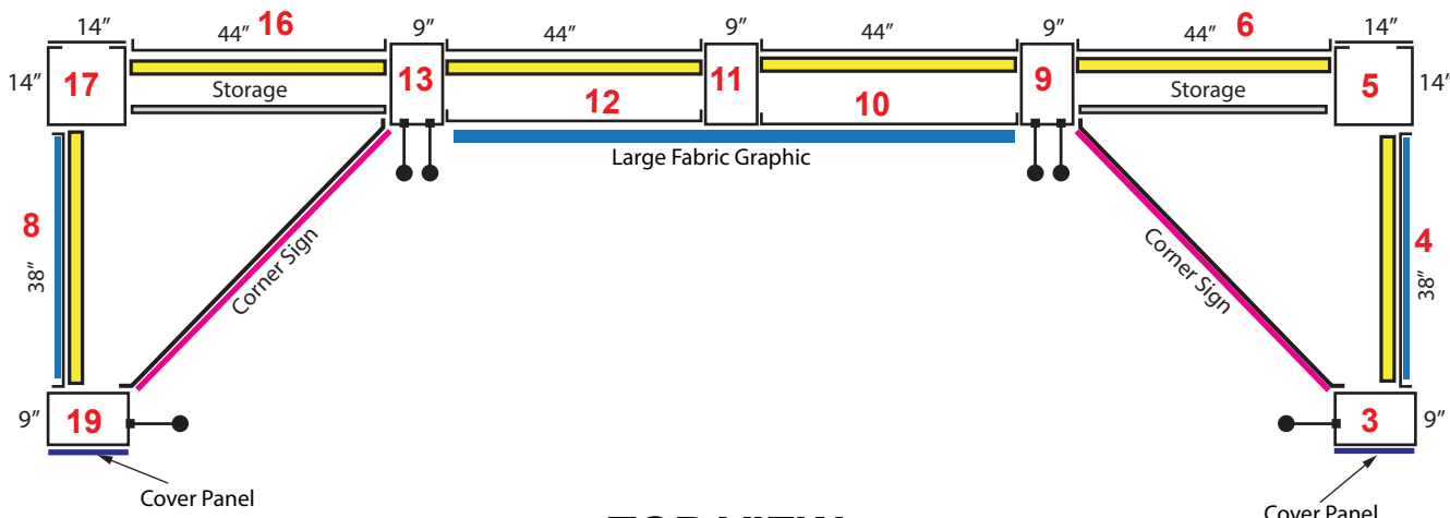
TOP VIEW Floor Plan: 20'x20'
