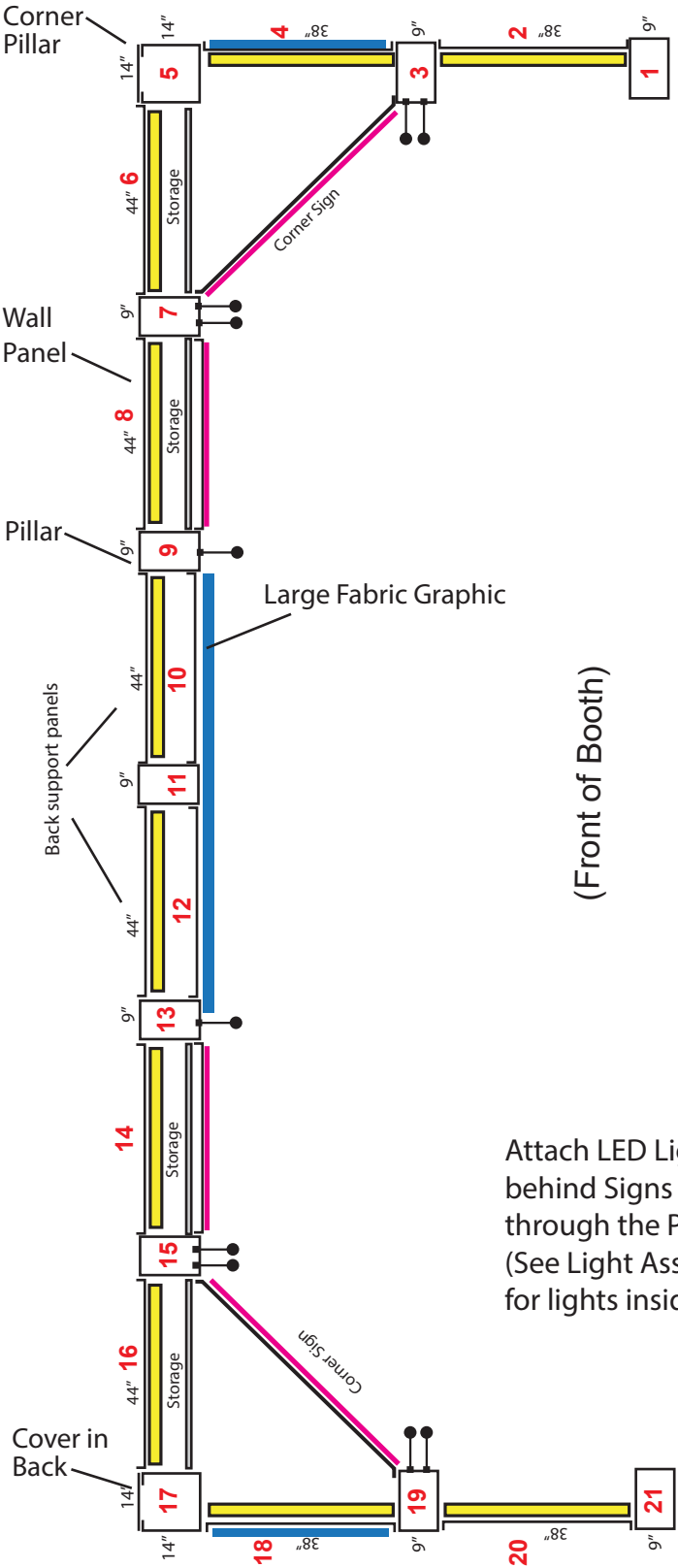
TOP VIEW Floor Plan: 10'x30'
