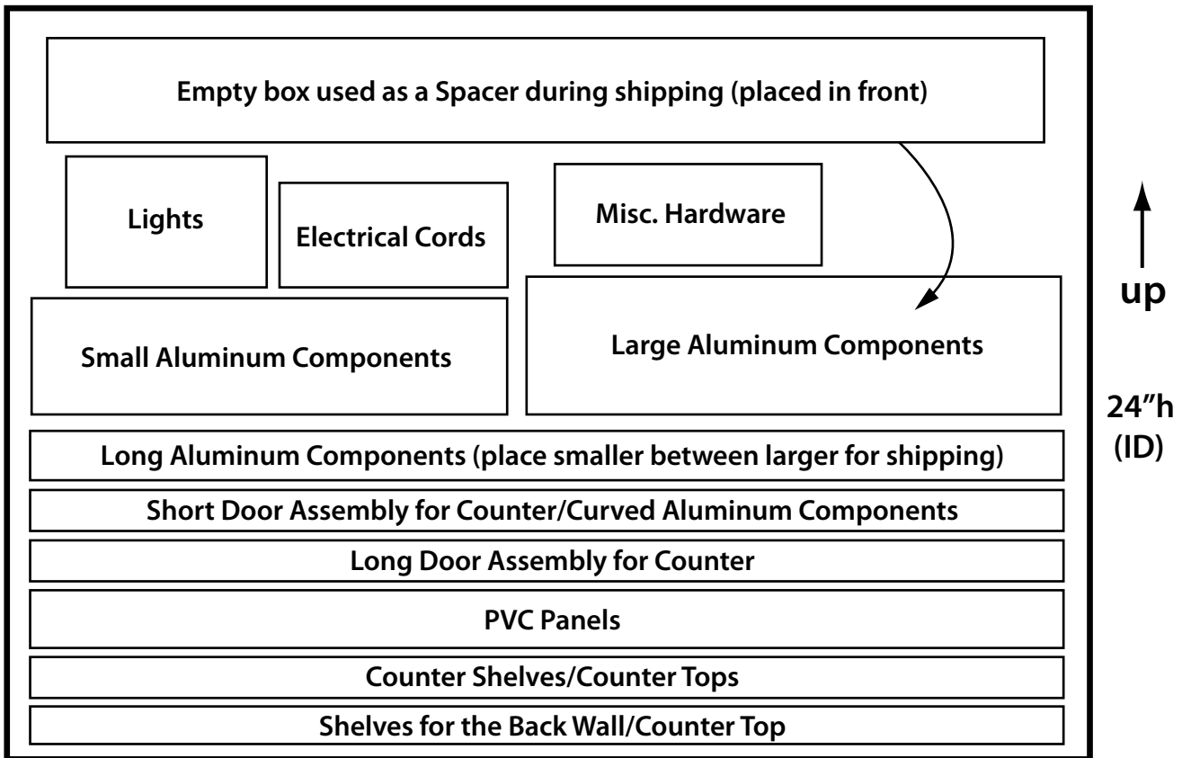
SIDE VIEW (not to scale)
