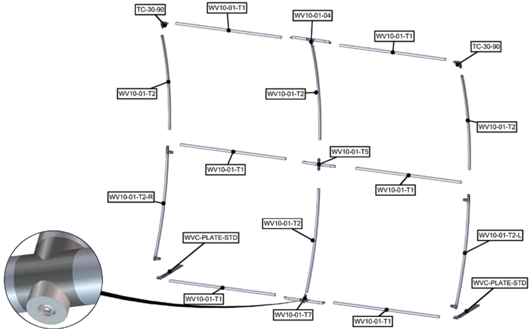
FabLite 10' Vertical Curve - FL10-VC
